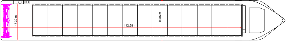
MAIN DECK
