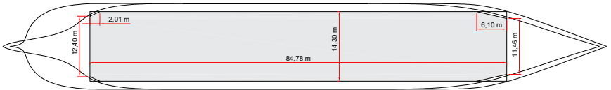
LOWER HOLD
